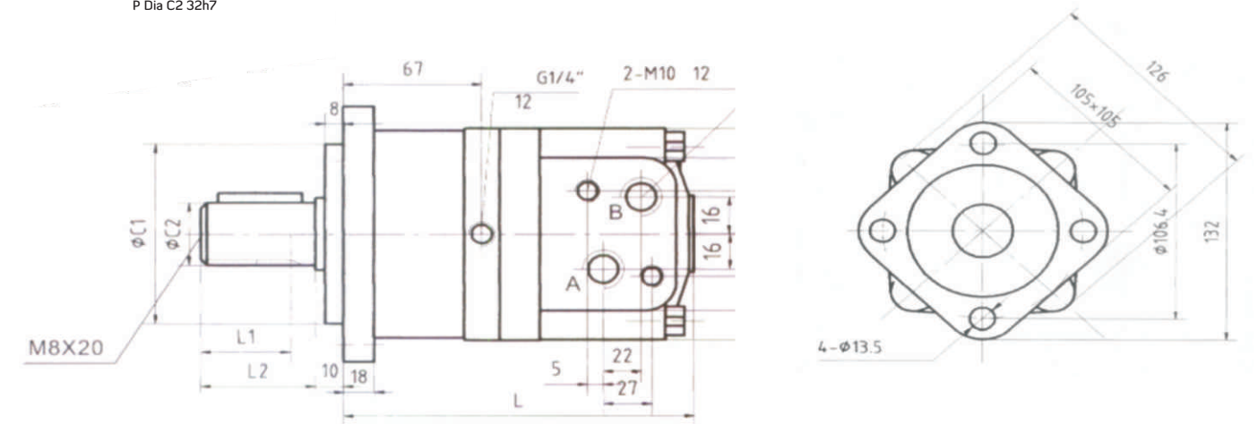
BM3-80-400P*A*Y BM3-80-400H*A*Y P Dia C2 32h7
