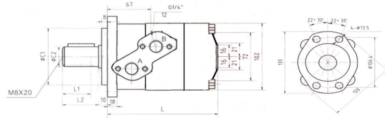
BMH-P Dia C2 32h7
