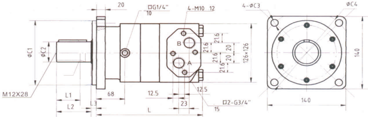
BM4 (BMT) P Dia C2 40h7 A125 Y
