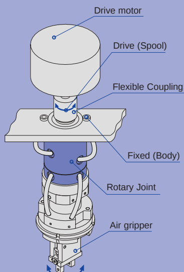
Example of spool drive
